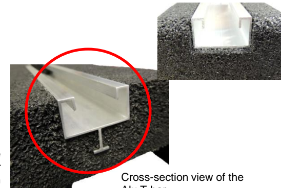
End view of the Alu T-bar
